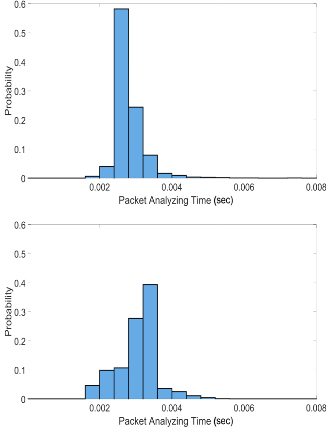
Fig. 9. The AD Processing Time per packet is shown at the Server when the SQF is used, and D = 2.7 ms. The average AD packet processing time is 2.97 ms and its variance is 0.0041 sec 2 when the attack occurs (above). The consequence of the Flood Attack (below) is to increase the AD average processing time of the AD per packet by just 10% to 3.28 ms, and a variance of 0.0023 sec 2 . This again demonstrates the effectiveness of the SQF.
