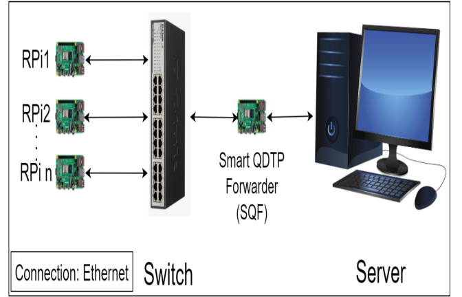
Fig. 6. The figure shows the modified system architecture where a Smart QDTP Forwarder (SQF) is placed before the Server, and acts as a traffic shaping interface between the Ethernet LAN and the Server. The effect of the SQF is to eliminate the paralyzing effect of the packet flood at the Server, buffering packets within the SQF, and forwarding the packets, so that AD processing and other work are conducted in a timely fashion.
