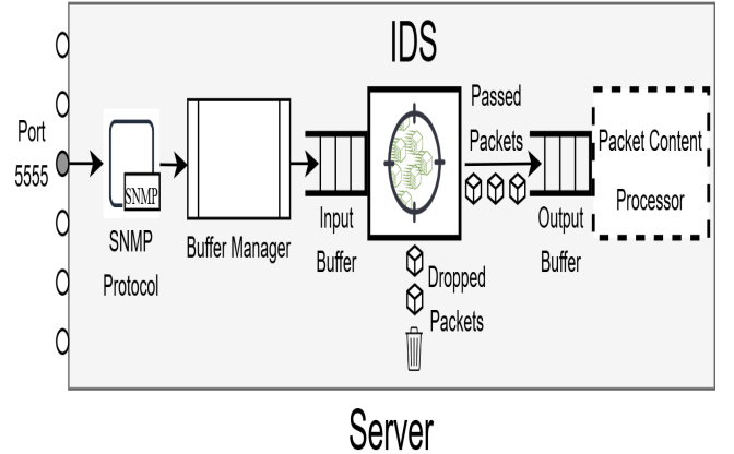
Fig. 2. The software at the Gateway Server includes the manager for the SNMP network, the attack detection system (AD) [15], as well as the software for processing the contents of incoming packets.
