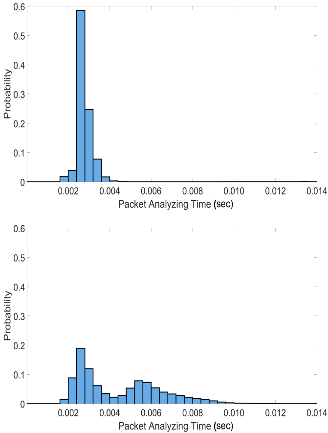
Fig. 4. In the figure that is above, one can observe the histogram of AD processing time per packet, as measured without an attack. It shows the average processing time of 2.98 ms (milliseconds), with a variance of 0.0055 \text{ ms}^2 . In the figure given below, an attack occurs and the AD packet processing time increases to the average value of 4.82 ms with 0.51 \text{ ms}^2 .
