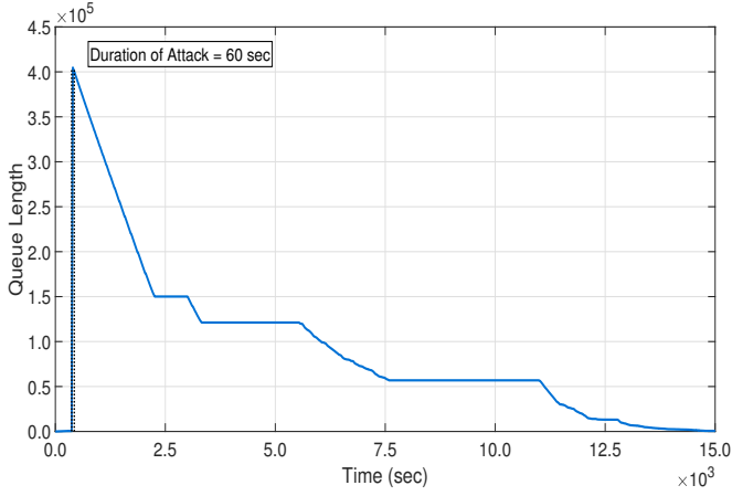
Fig. 3. The queue length shown along the y -axis (number of packets) at the Server input prior to the AD, shown as it varies over time ( x -axis in seconds) at the Server input, prior to processing by the AD module, for a 60 – seconds UDP Flood Attack that was launched by a Raspberry Pi in Figure 1. The queue length rises rapidly to 400,000, and the Server congestion then lasts far longer than the attack itself, i.e. up to several hours, because of Server paralysis which delays AD processing, as seen in the AD processing times of Figure 5.
