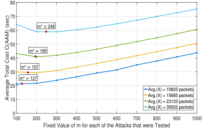
Fig. 14. Experimental graph (when both the x and y coordinates are linear, i.e. not logarithmic) of the Average Total Cost C(AAM) over thirty independent experiments for \frac{\beta}{\alpha} = 0.05 , plotted against the parameter m . We see that the average cost depends on m , and confirms that the theoretically predicted m^* provides a useful value of cost minimization.
